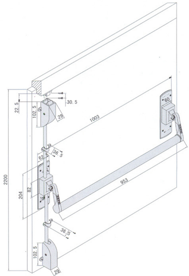
VR-220P 下压式安全门锁（含天地插销） 静电粉体涂装 Crossbar Exit Device — Powder Electrostatic Coating (With Flush Bolt)
